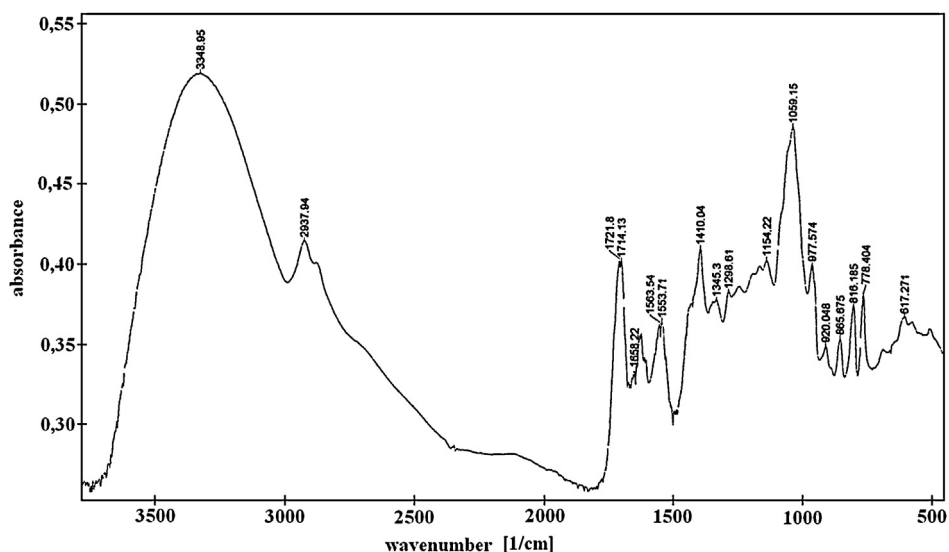
Fig. 4. FTIR spectrum of 1-O-acryloyl-D-fructose.
